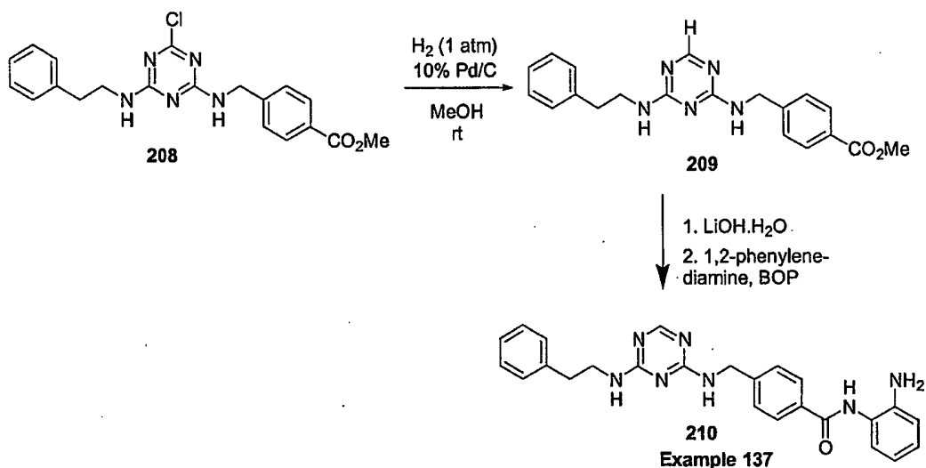
Scheme 26
